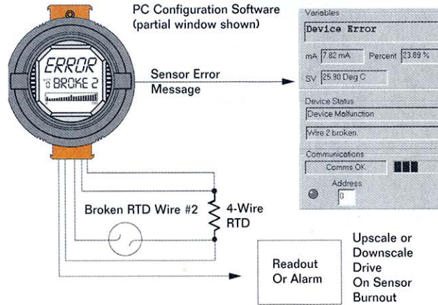
FIGURE 5. Some transmitters provide specific fault messages that speed diagnosing the exact sensor problem.
